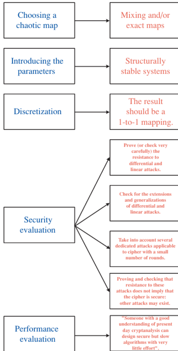
Figure 2-38 A Procedure for a design of a chaos-based block-encryption algorithm [41]
